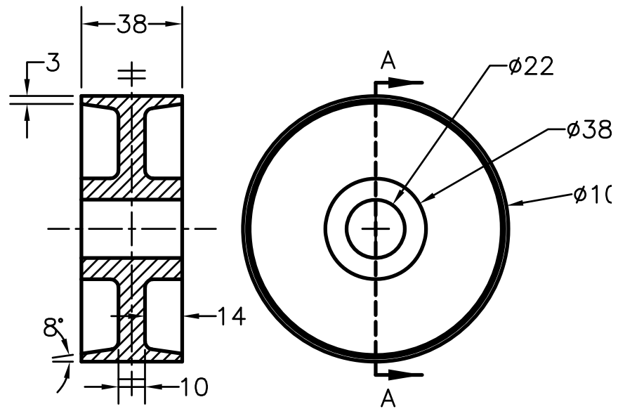
SECTION A-A WHEEL
