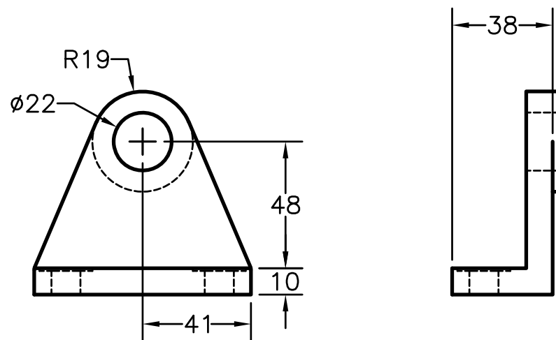
AXLE SUPPORT
