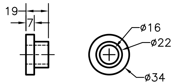
BUSHING
