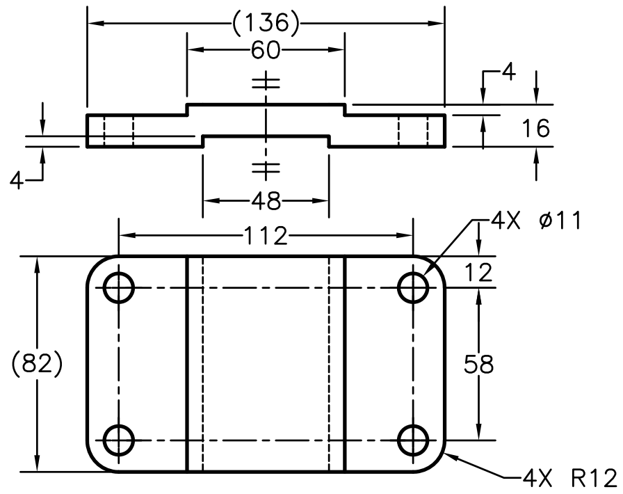
TOP PLATE
